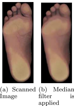
Figure 7: Input Images
